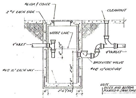
GREASE TRAP NO SCALE
