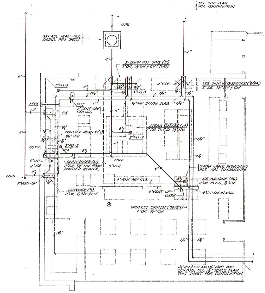
KITCHEN PLAN - PLUMBING SCALE: 1/4" = 1'-0"
